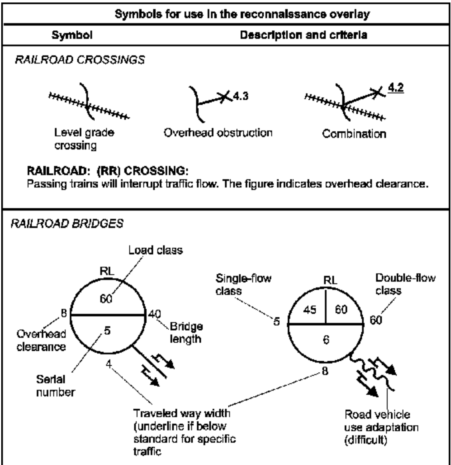
Figure 9-1. Reconnaissance overlay symbols (continued).
